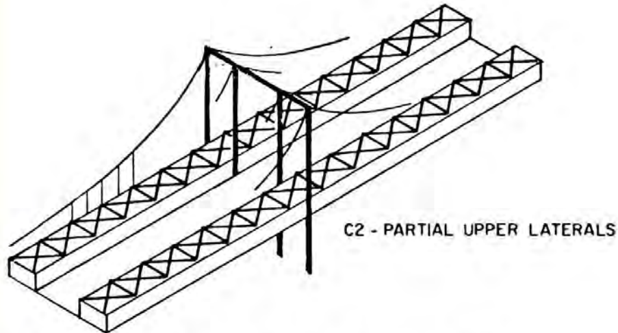
Figure 3. Manhattan Bridge stiffening system layout
