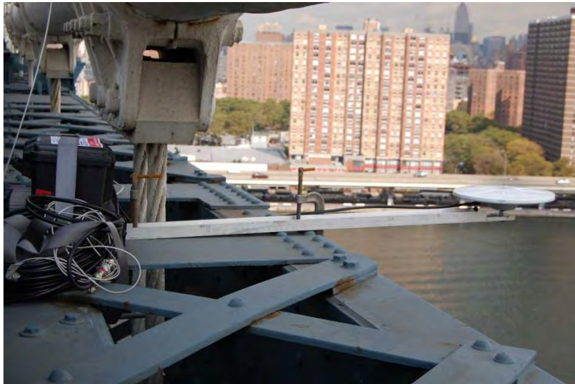
Figure 4. GPS receiver mounted on Manhattan Bridge
