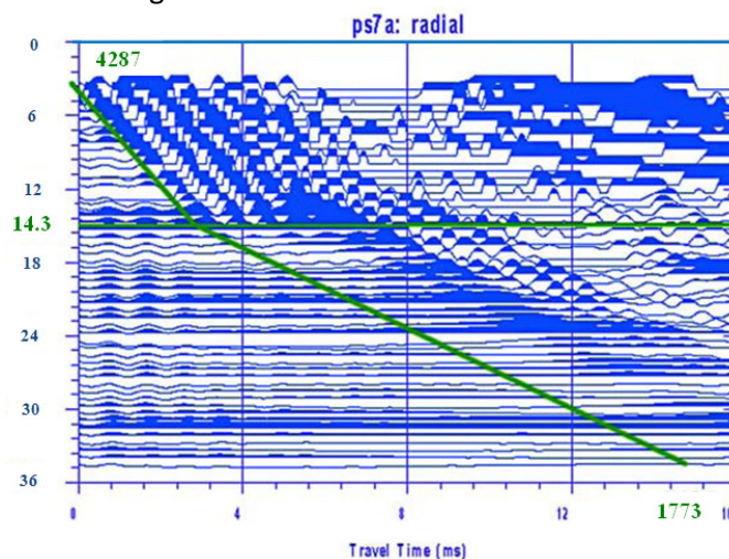
Figure 2 The figure to the left shows PS results from tests performed on a concrete pile in saturated soils. The bottom of the concrete pile is identified at 14.3m where the compressional wave velocity changes from 4287 m/sec (velocity of concrete) to a velocity of 1773 m/sec (velocity of water).
