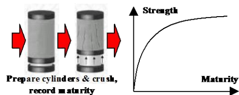
Figure 3 – Measuring Maturity/Strength Insitu
