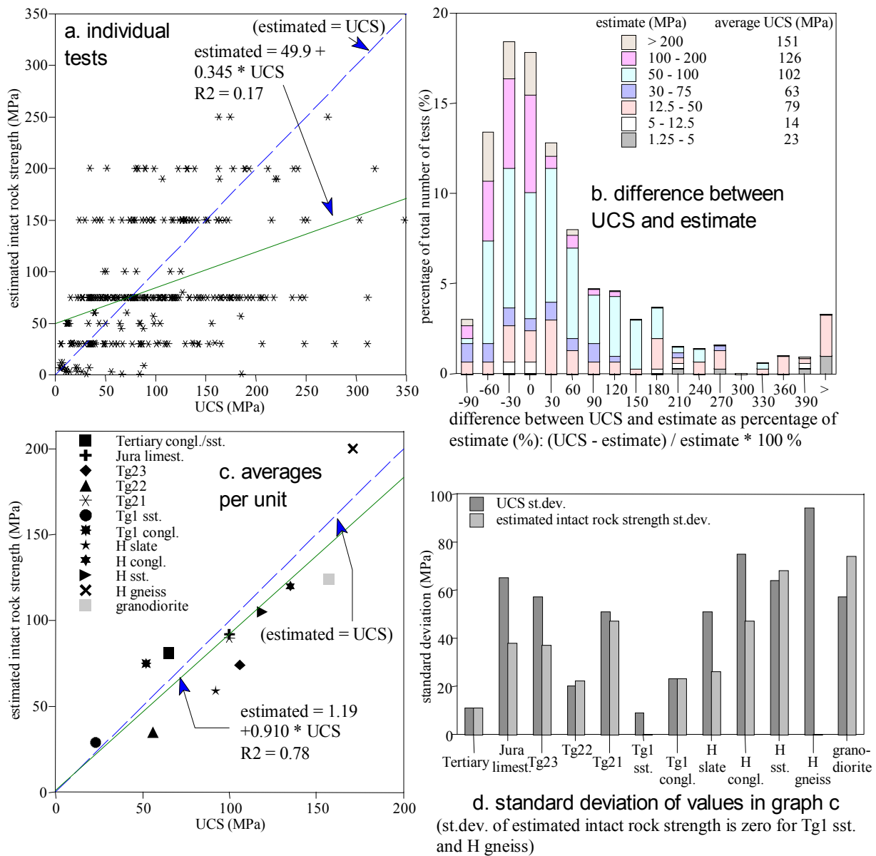
Figure 1. Estimated intact rock strength vs. strength values determined by UCS tests. (The dashed lines in A and C indicate the relation if estimated strength equals UCS strength.) (Number of UCS tests: 941)
