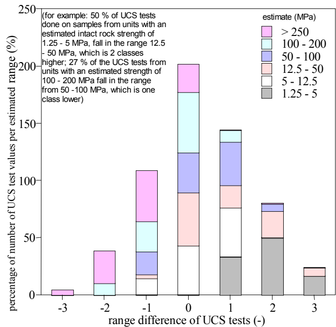
Figure 4. Percentage of UCS test values falling in a range different from the estimated value.
