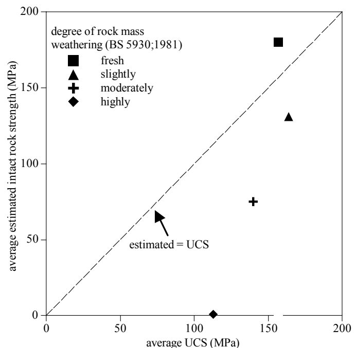
Figure 2. Average estimated intact rock strength vs. average UCS for granodiorite units with various degrees of rock mass weathering.
