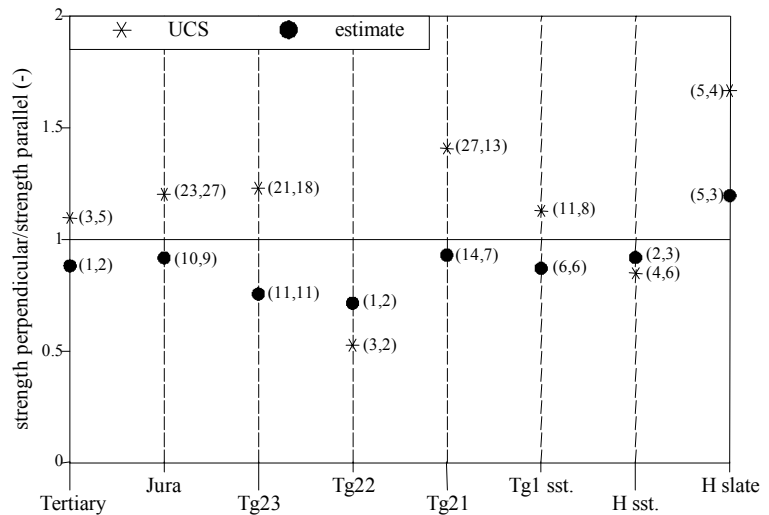
Figure 5. Ratio of average intact rock strength perpendicular over average intact rock strength parallel for UCS and field intact rock strength estimate per unit (values in brackets are the number of UCS tests respectively estimate)
