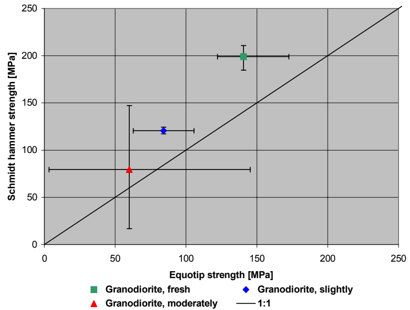
Figure 3. UCS strength estimated with in-situ field tests Equotip and Schmidt hammer; crosses indicate spread in measurements.
